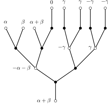
Figure 3: An example NAND tree to illustrate Lemmas 3 and 4. As in Figure 1, a vertex is filled or not according to whether it evaluates to 1 or 0, respectively. The amplitudes \langle v | a \rangle of a zero-energy eigenstate |a\rangle for the adjacency matrix H are also labeled, with \alpha, \beta, \gamma free variables, assuming h_{pv} = 1 for every edge (p, v) . The amplitudes of the neighbors of any vertex sum to zero. The existence of such an |a\rangle is promised by Lemma 4. As required by Lemma 3, \langle v | a \rangle = 0 if \bar{\Lambda}(v) = 1 , so vertices evaluating to 1 are not labeled.
